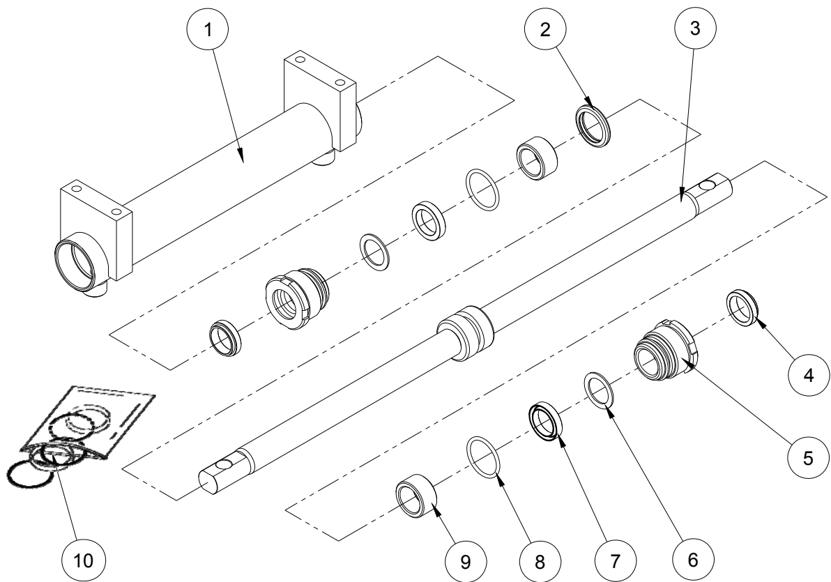
Figure 4-3 Steer Cylinder
