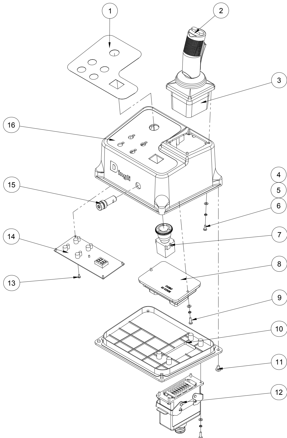
Figure 3-5 Platform Control
