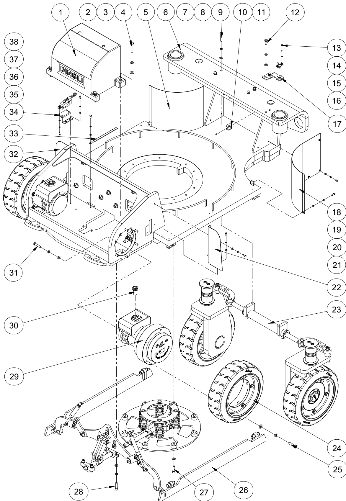
Figure 1-2 Chassis Assembly
