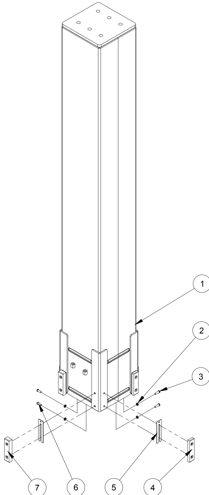
Figure 2-13 Mast 5 Assembly (AMWP10-8100)
