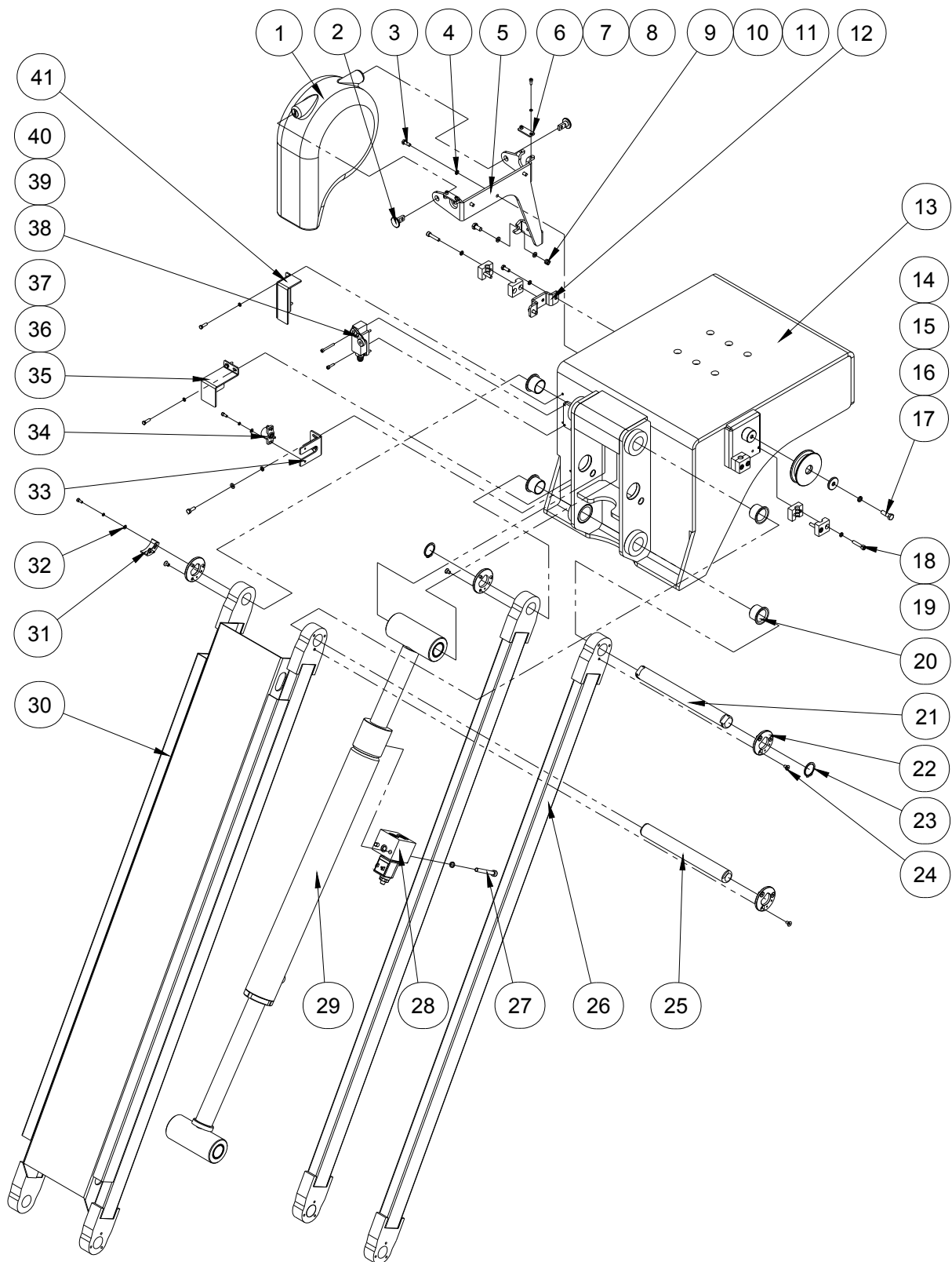
Figure 3-3 Jib Assembly
