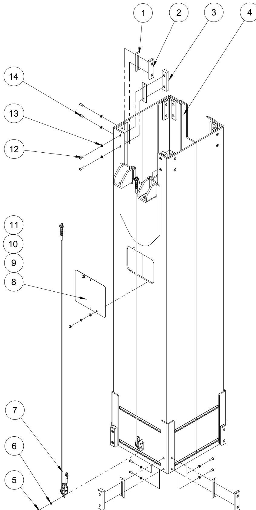
Figure 2-4 Mast 2 Assembly
