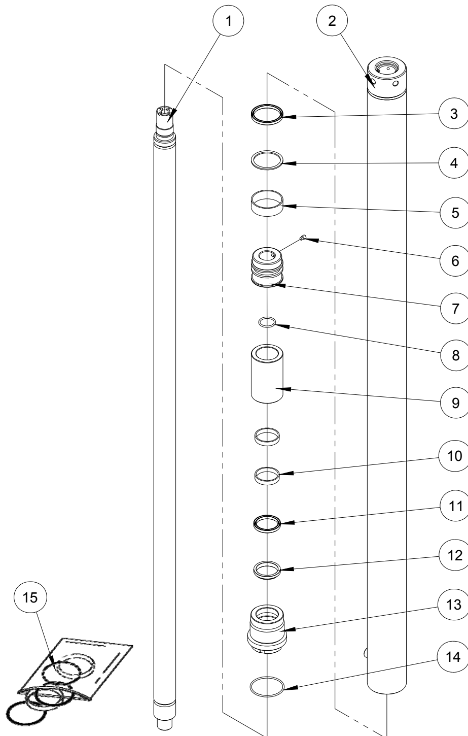
Figure 4-1 Lift Cylinder
