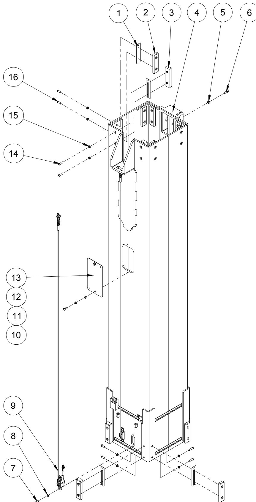
Figure 2-6 Mast 4 Assembly (AMWP11.5-8100)
