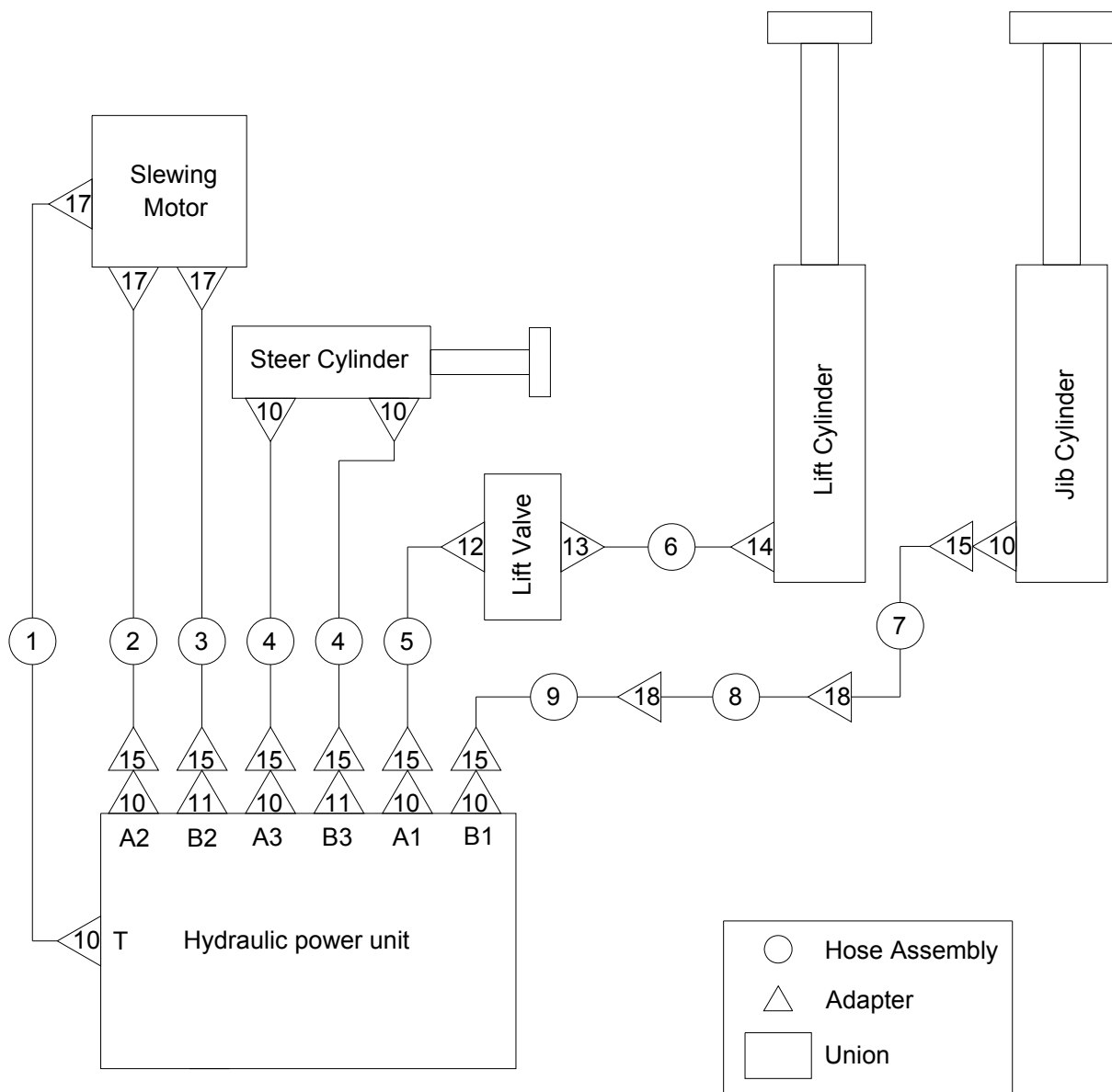
Figure 4-4 Hydraulic Hoses and Fittings
