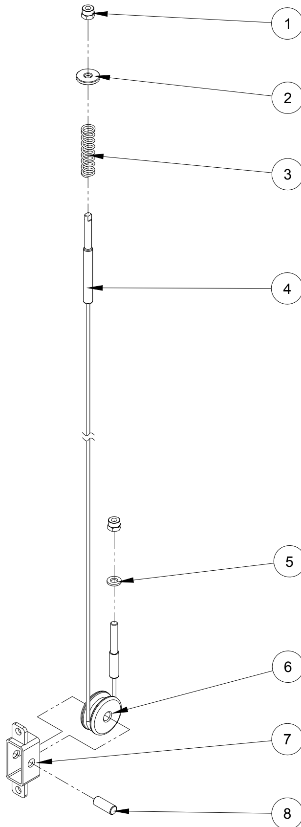
Figure 2-9 Cable Assembly
